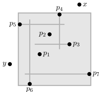
Figure 2: The points p_1, \dots, p_7 form a proper pin sequence and the gray box denotes \text{rect}(p_1, \dots, p_7) . The point x satisfies the externality and separation conditions for this pin sequence and thus could be chosen as p_8 ; y , however, fails the separation condition.
