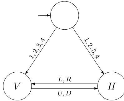
Figure 7: An automaton that accepts the language of strict pin words ( V and H are accept states).
