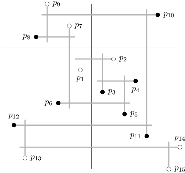
Figure 6: The proper pin sequence p_1, \dots, p_{15} shown corresponds to the strict pin word w = 3RDRDLULURDLDRD . The filled points correspond to the pin word u = 4RDL21DL , the permutation corresponding to this word, i.e., the permutation order isomorphic to the filled points, is 27453618.
