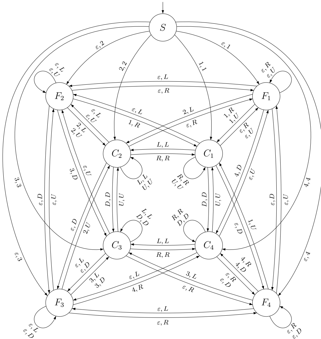
Figure 8: The transducer that produces all strict pin words containing the input pin word.
