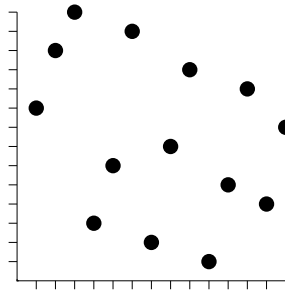
Figure 1: The plot of a simple permutation.
