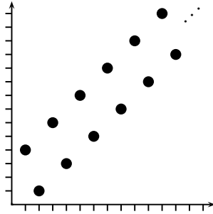
Figure 9: A plot of the increasing oscillating sequence.
