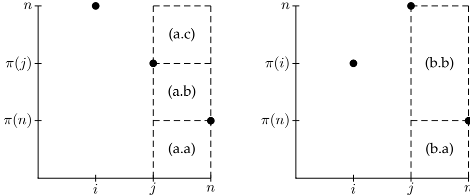
Figure 5: The two situations in the proof of Proposition 2.4.
