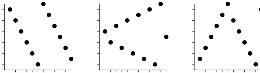
Figure 3: From left to right: a parallel alternation (which in this case happens to be simple), a wedge simple permutation of type 1, and a wedge simple permutation of type 2.
