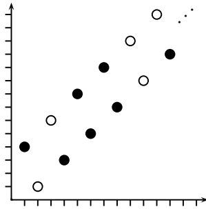
Figure 10: The filled points show the embedding of 2153647, with rank encoding 1020100, given by the proof of Proposition 6.2.
