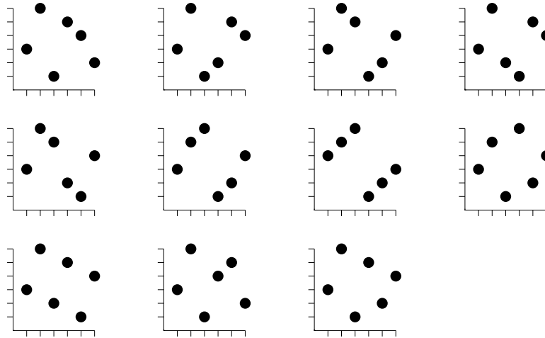
Figure 11: The basis elements of length 6 for the pin class (up to symmetry).
