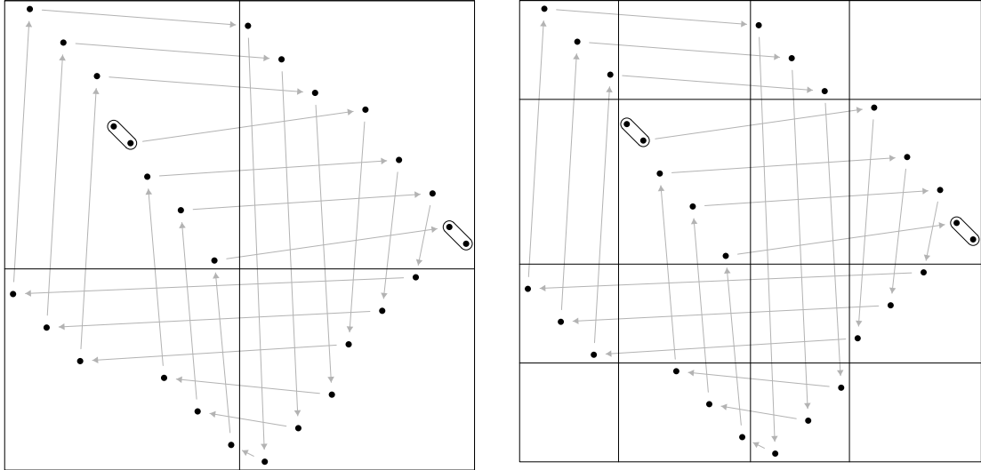
Figure 3: The permutation on the left is a permutation constructed by our algorithm to lie in \text{Prof} \begin{pmatrix} 1 & 1 \\ 1 & -1 \end{pmatrix} . On the right, we have a permutation constructed by our algorithm to lie in the profile class of
