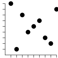
Figure 2: The plot of the skew-merged permutation 917456328.
