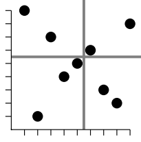
Figure 3: A gridding of the skew-merged permutation 917456328.
