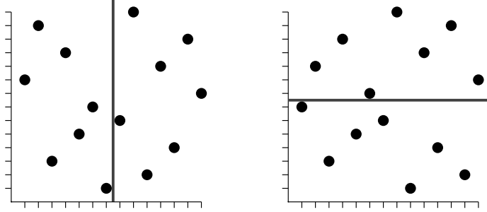
Figure 6: A horizontal alternation (left) and its inverse, a vertical alternation (right).
