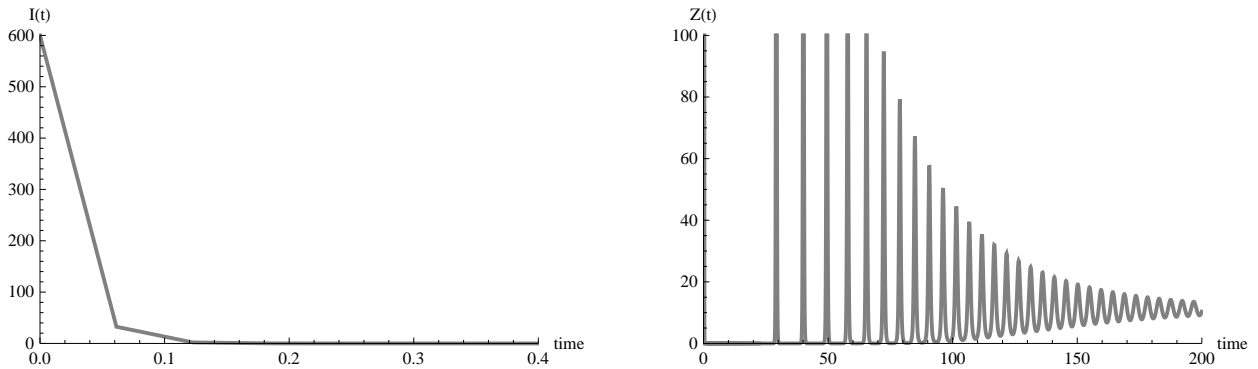
Figure 4: The left figure shows that the number infected with human influenza tends to zero. The right figure shows that the pandemic strain become established. Parameters are as in Table 5 and \beta_Z = 0.00277 , \nu_Z = 60 , and \mathcal{R}_2 = 3 . In the above simulation \rho = \beta_J = 0 and Z(0) = 0.00001 , \nu_J = 0.1 * 365 .
