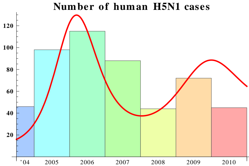
Figure 2: Number of human cases of H5N1 per year as given by WHO [45]. The red curve is the predictions of the model.
