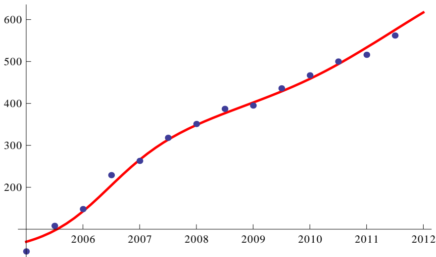
Figure 3: Commutative number of human cases of H5N1 as given by WHO [45]. The red curve is the predictions of the model. Time is measured in years since 01/01/2005. Data points correspond to the cases in the first or second half of year.
